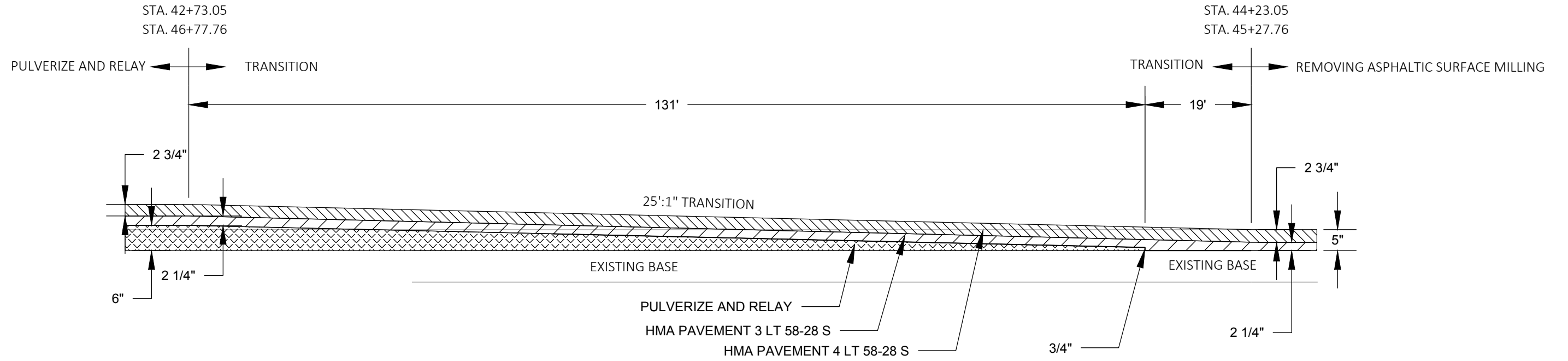
PULVERIZE AND RELAY TO REMOVING ASPHALTIC SURFACE MILLING TRANSITION
